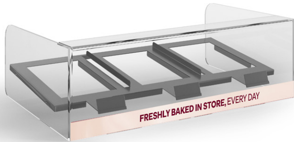
PSIT SINGLE TIER PASTRY STAND WITH SNEEZE SCREEN 629 W x 400 D x 200 H mm (200 W x 380 D CHEFS TABLE TRAYS REQUIRED) FOR USE ON ALL VICTOR SOTF STORES WITH 2 FRIDGES USED ON SECOND FRIDGE CLOSEST TO THE TILL ALL VERSIONS OF: F12A, F15A, F18AC/CA
